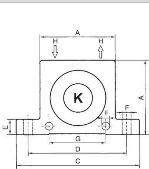
Pneumatic Vibrator K series Ball Vibrator
