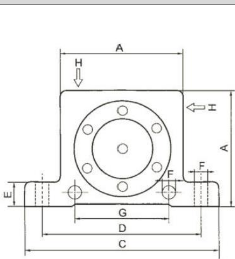
Pneumatic Vibrator R series Roller Vibrator
